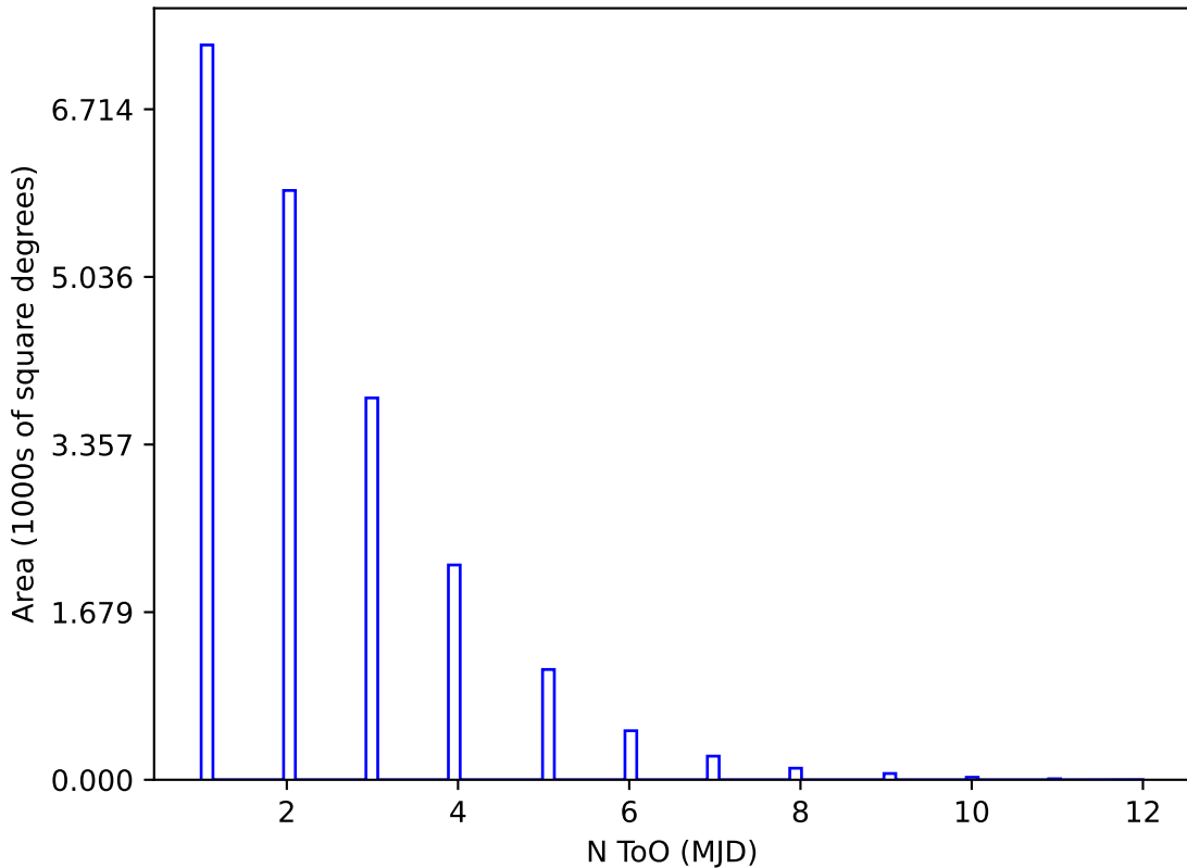
too_100_1v3.4_10yrs g and note like ToO%: N ToO
