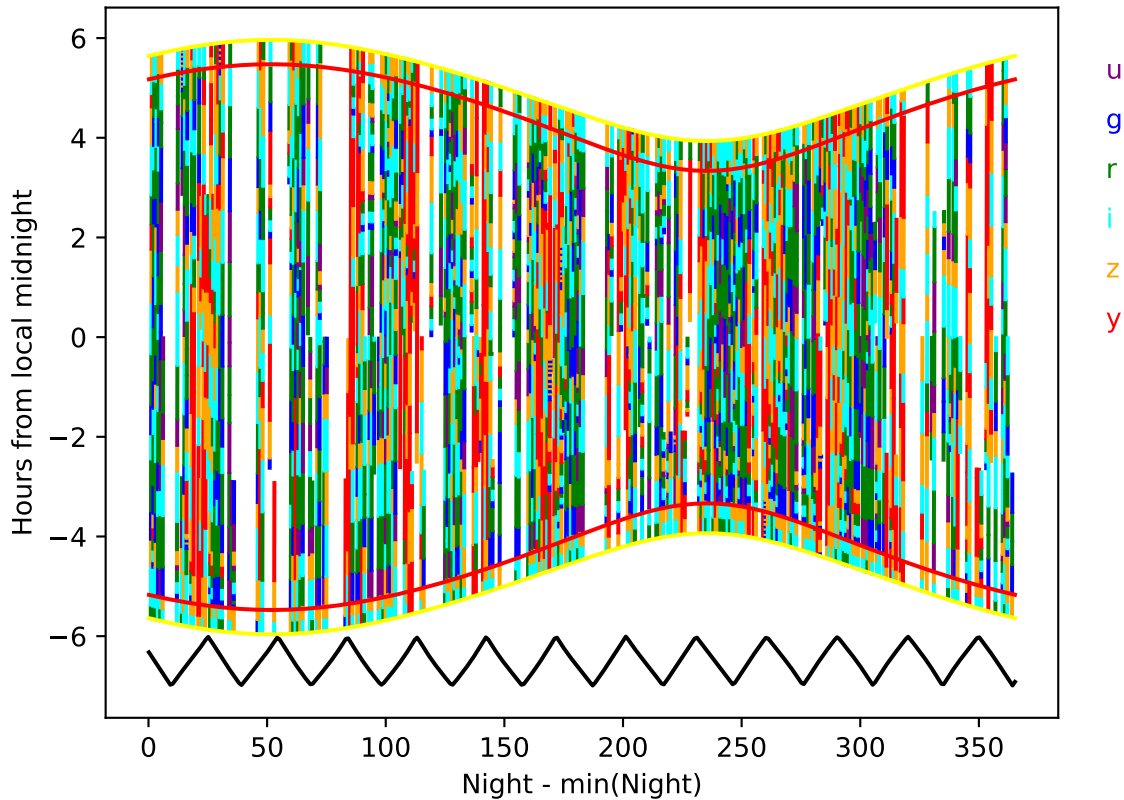
too_100_1v3.4_10yrs year 7-8: Hourglass
