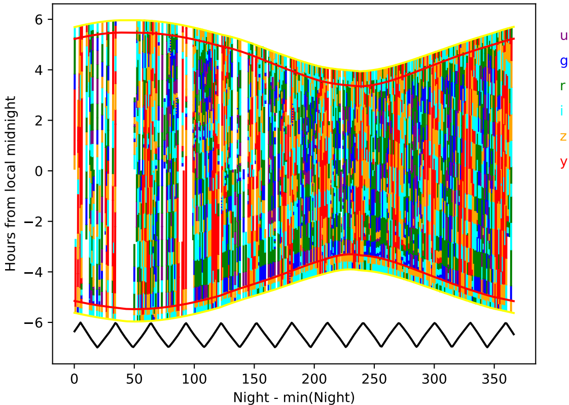
too_100_1v3.4_10yrs year 6-7: Hourglass
