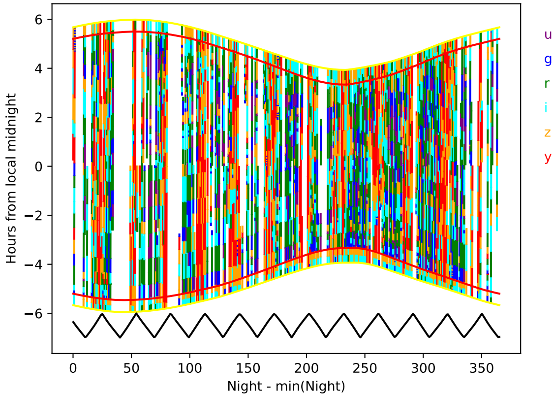
too_100_1v3.4_10yrs year 4-5: Hourglass
