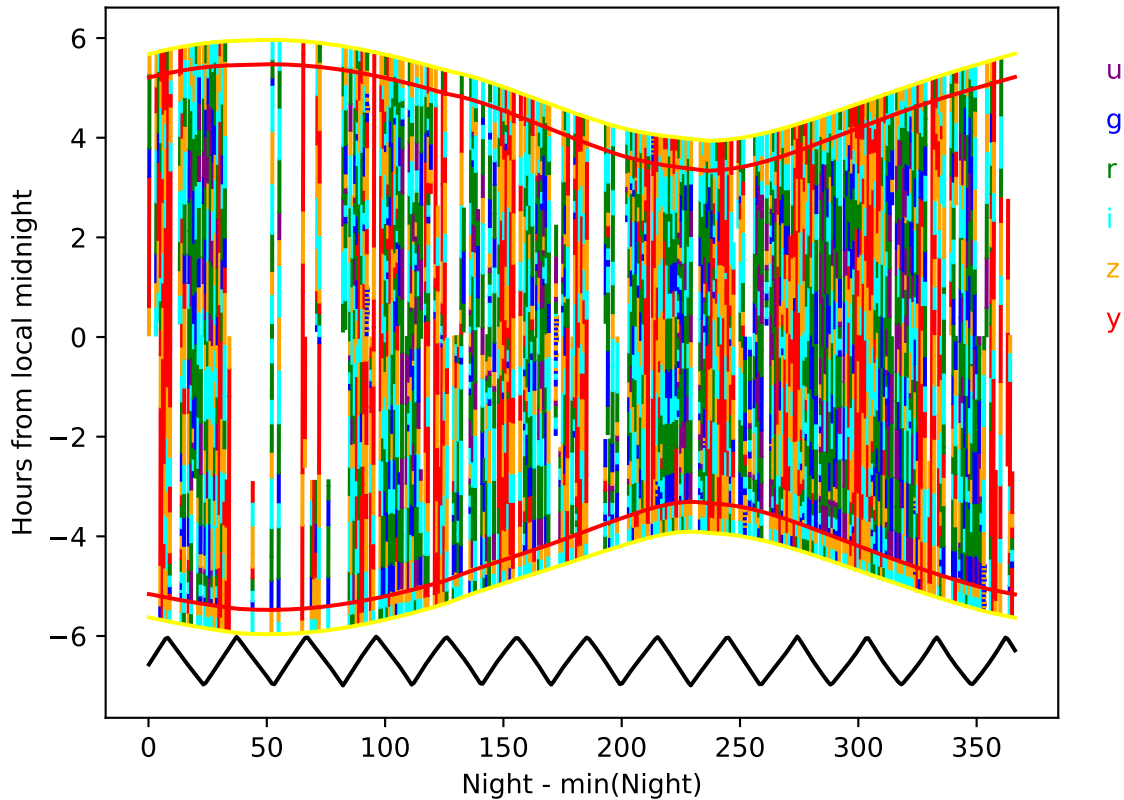
too_100_1v3.4_10yrs year 3-4: Hourglass
