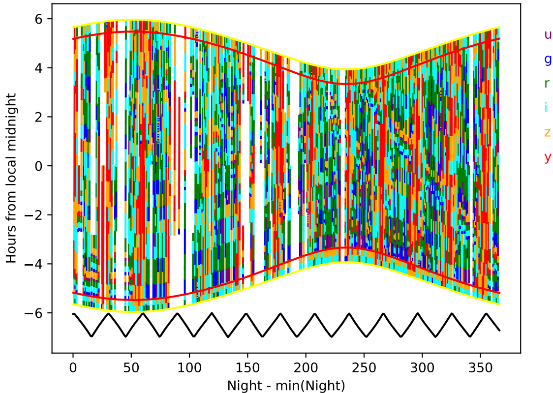
too_100_1v3.4_10yrs year 1-2: Hourglass
