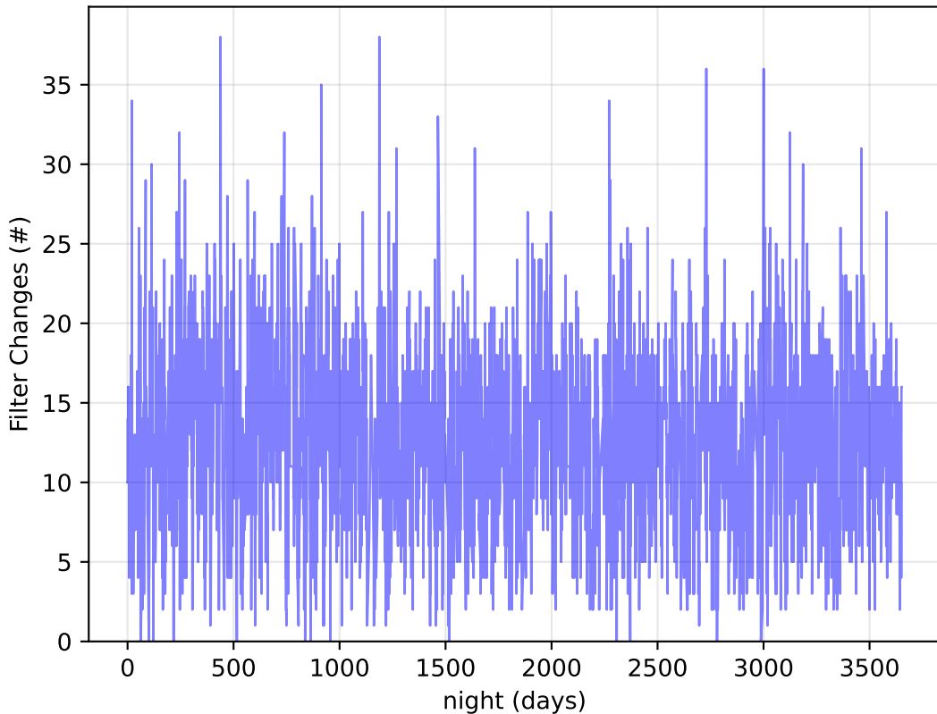
too_100_1v3.4_10yrs : Filter Changes
