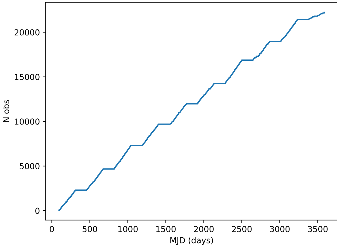
too_100_1v3.4_10yrs note like DD:ECDFS%: Cumulative
