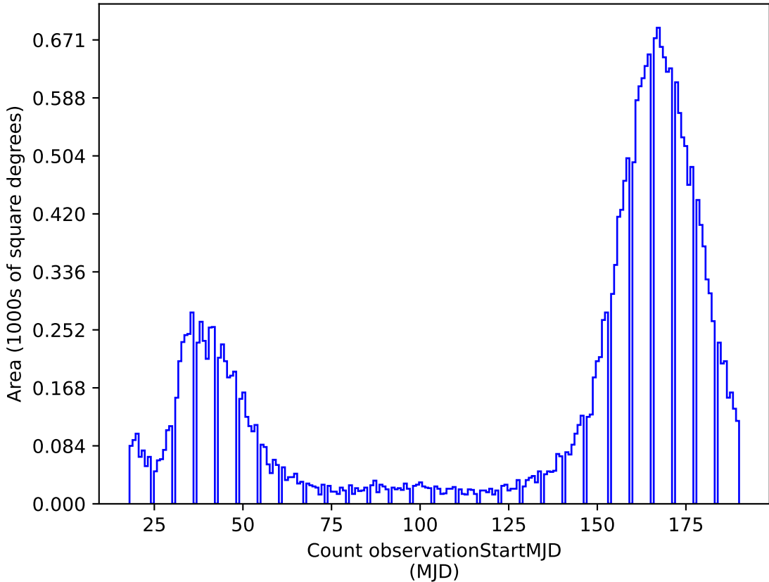
too_100_1v3.4_10yrs z: Count observationStartMJD
