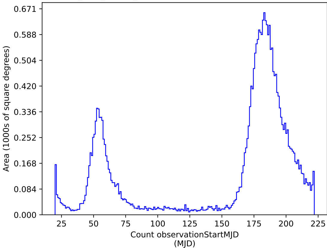
too_100_1v3.4_10yrs r: Count observationStartMJD
