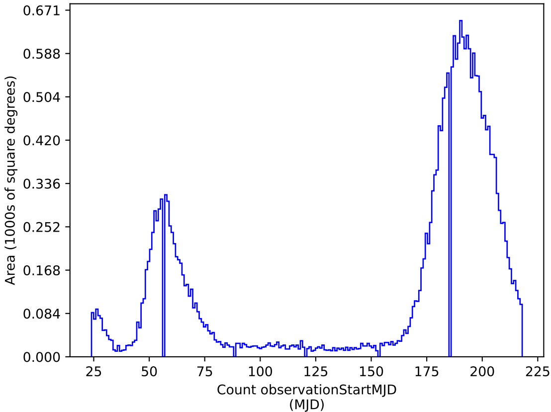
too_100_1v3.4_10yrs i: Count observationStartMJD
