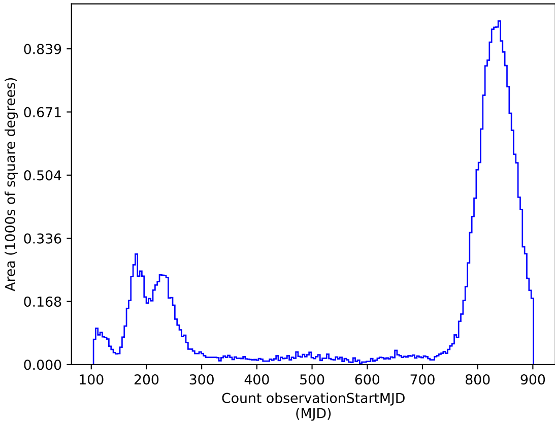
too_100_1v3.4_10yrs : Count observationStartMJD
