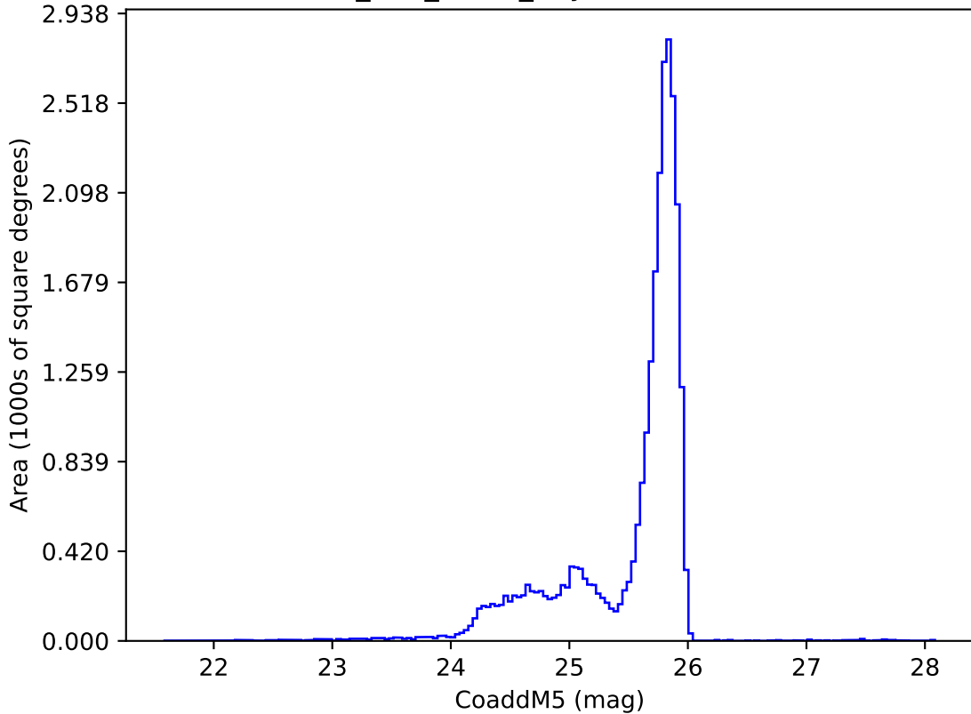
too_100_1v3.4_10yrs z: CoaddM5
