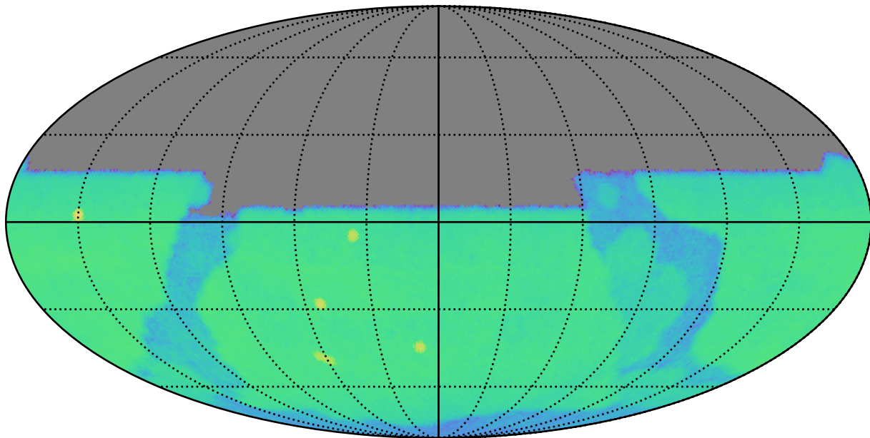
too_100_1v3.4_10yrs u: CoaddM5
