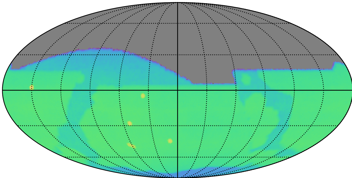
too_100_1v3.4_10yrs r: CoaddM5
