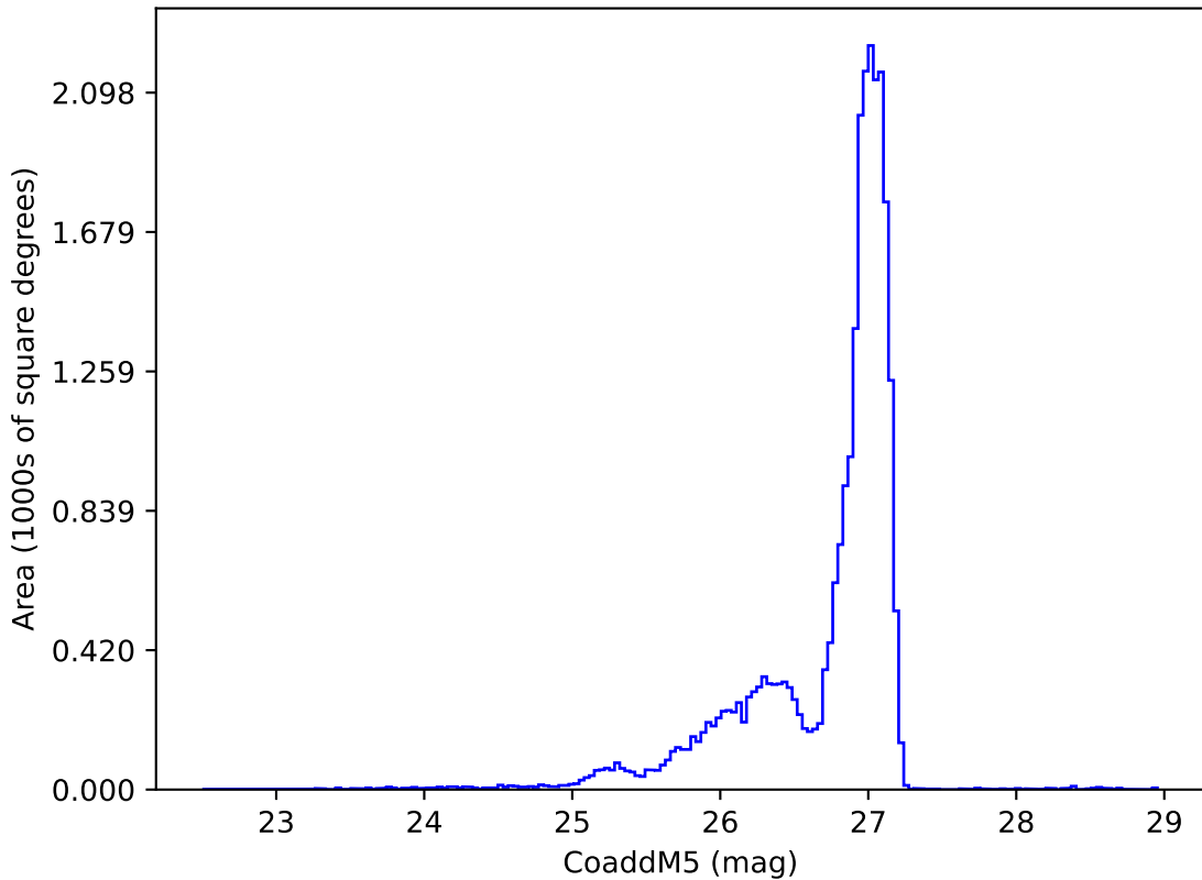
too_100_1v3.4_10yrs r: CoaddM5
