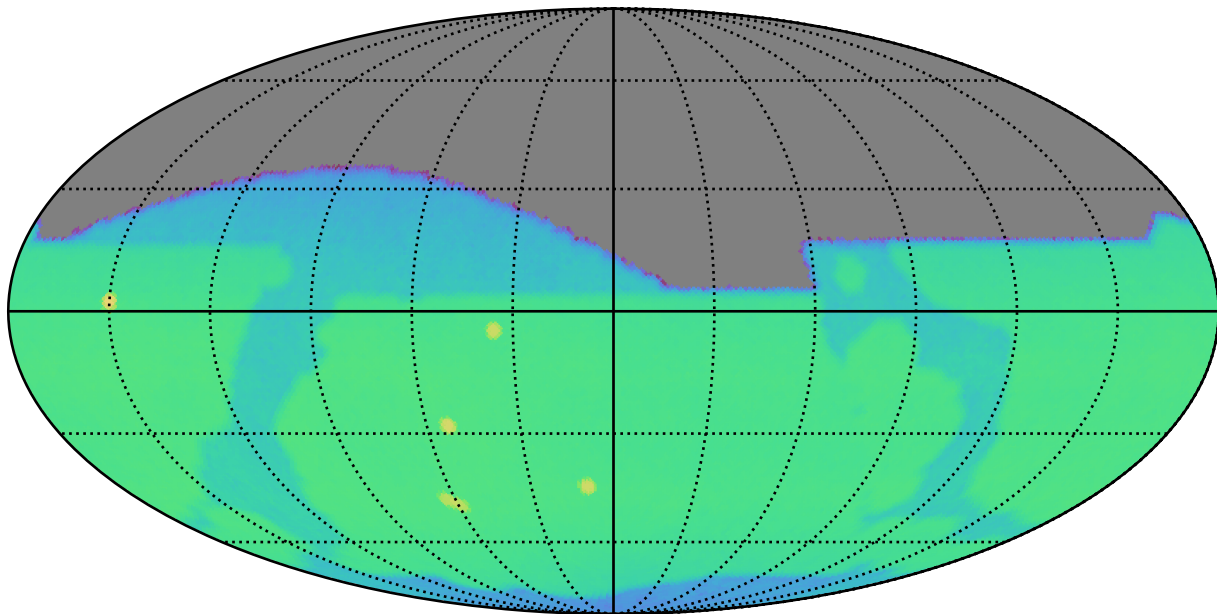
too_100_1v3.4_10yrs i: CoaddM5
