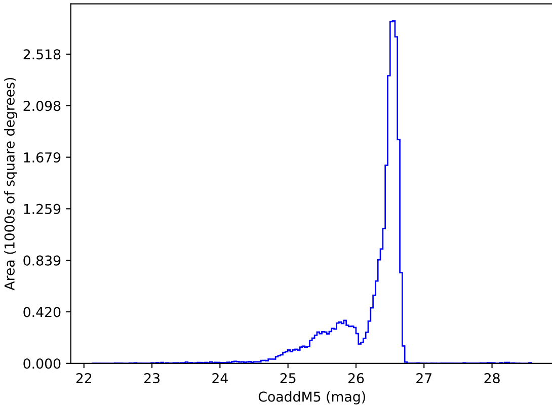
too_100_1v3.4_10yrs i: CoaddM5
