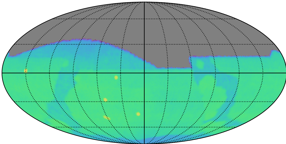
too_100_1v3.4_10yrs g: CoaddM5
