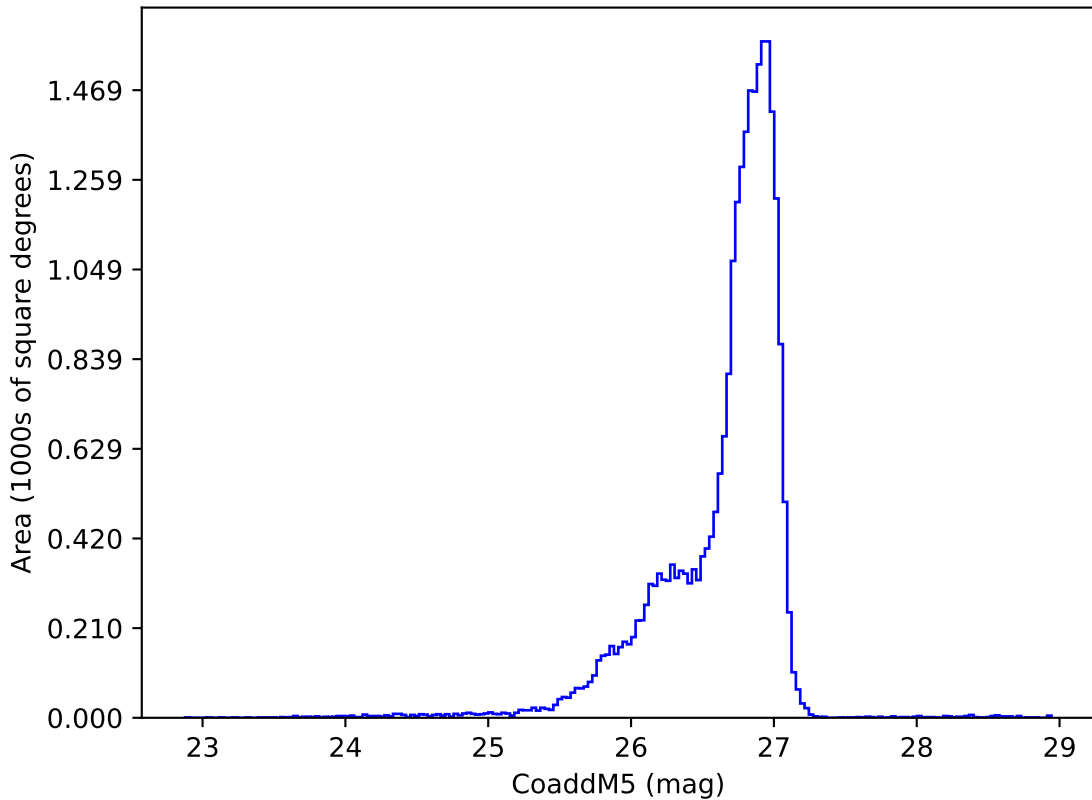
too_100_1v3.4_10yrs g: CoaddM5
