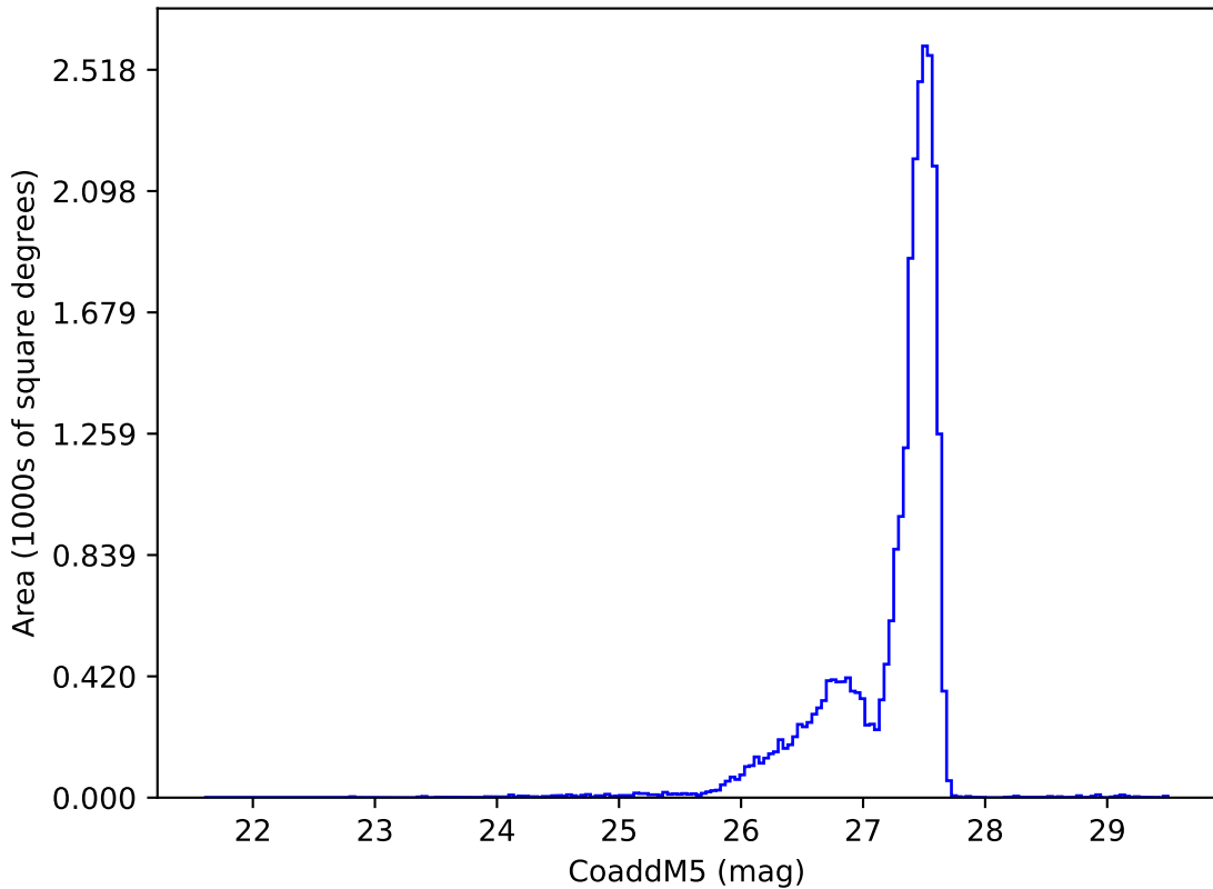
too_100_1v3.4_10yrs : CoaddM5
