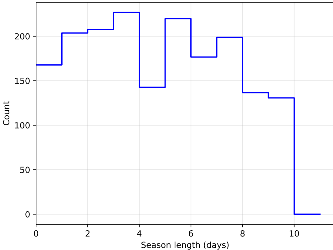
too_100_1v3.4_10yrs DD:WFD all bands: SeasonLength
