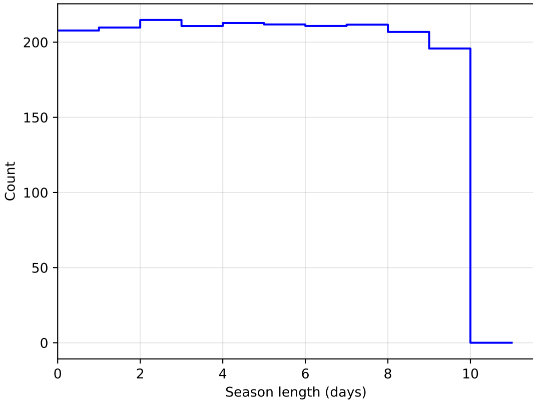
too_100_1v3.4_10yrs DD:EDFS all bands: SeasonLength
