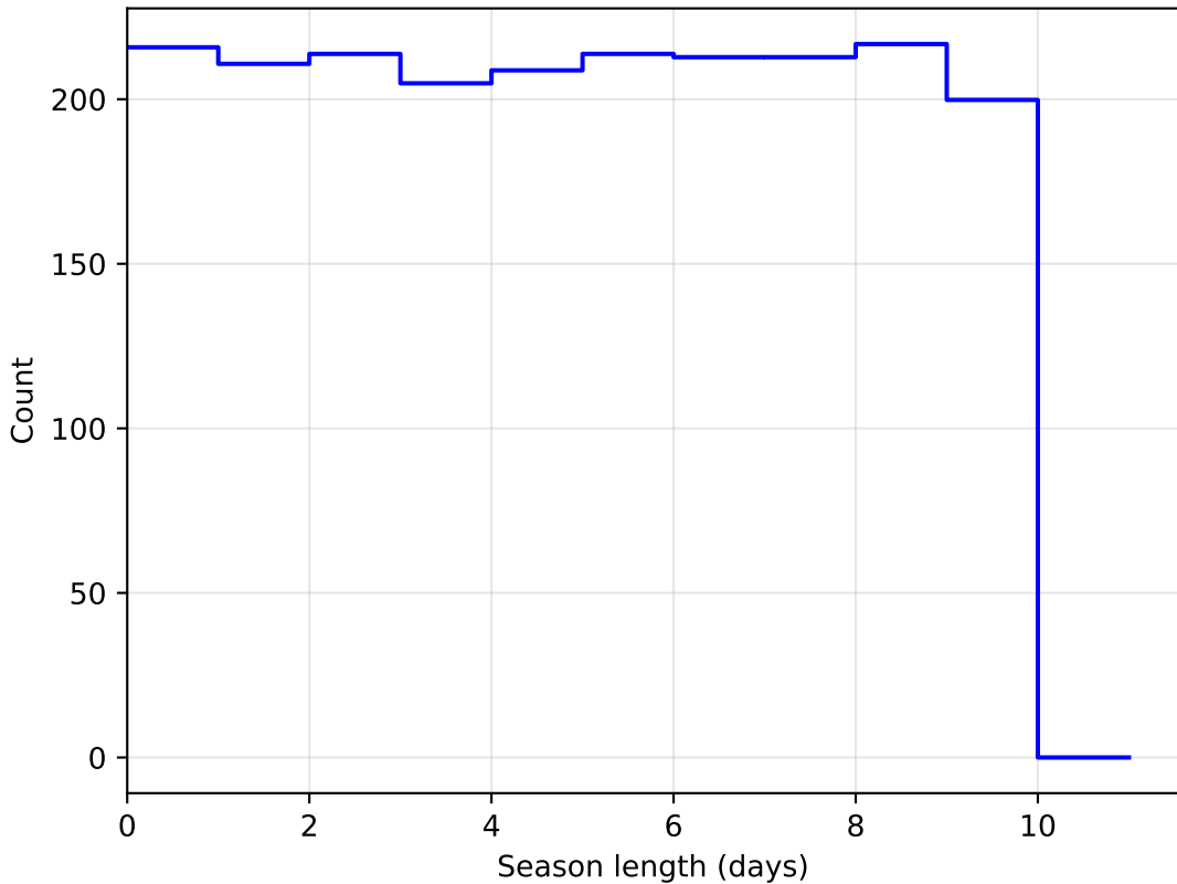
too_100_1v3.4_10yrs DD:ECDFS all bands: SeasonLength
