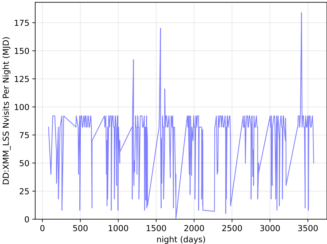
too_100_1v3.4_10yrs all bands: DD:XMM_LSS Nvisits Per Night
