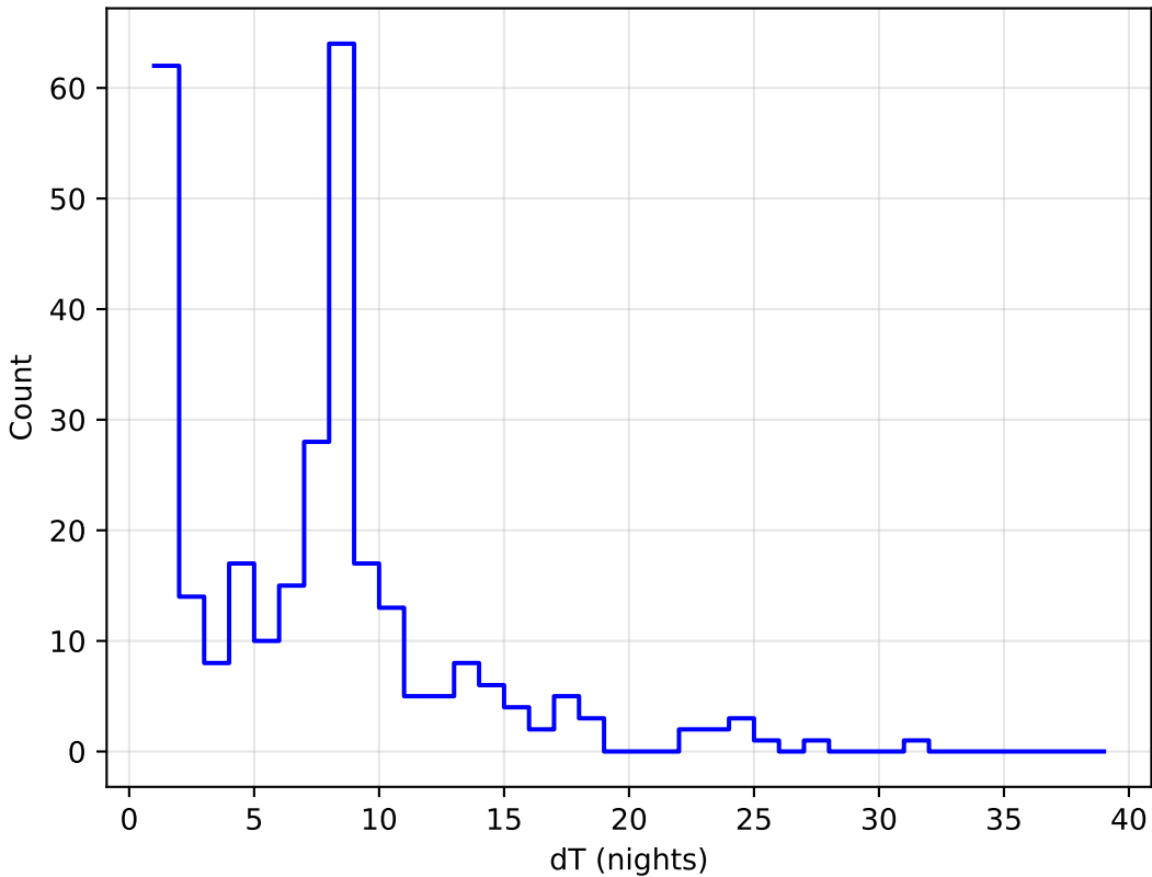
too_100_1v3.4_10yrs all bands: DD:XMM_LSS Delta Nights Histogram
