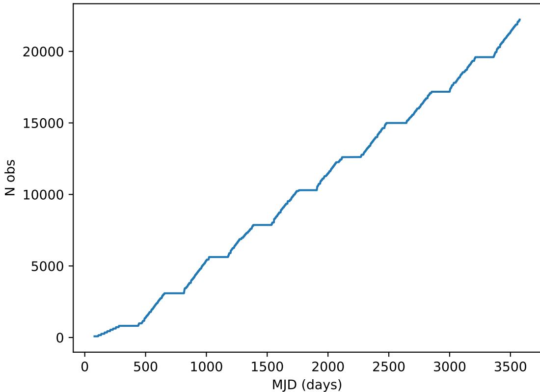
too_100_1v3.4_10yrs all bands: DD:XMM_LSS Cumulative NVisits
