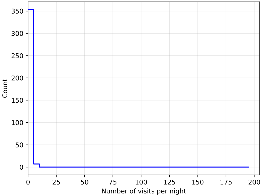
too_100_1v3.4_10yrs all bands: DD:WFD NVisitsPerNight
