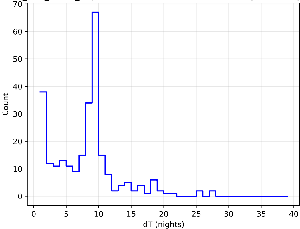
too_100_1v3.4_10yrs all bands: DD:ELAISS1 Delta Nights Histogram
