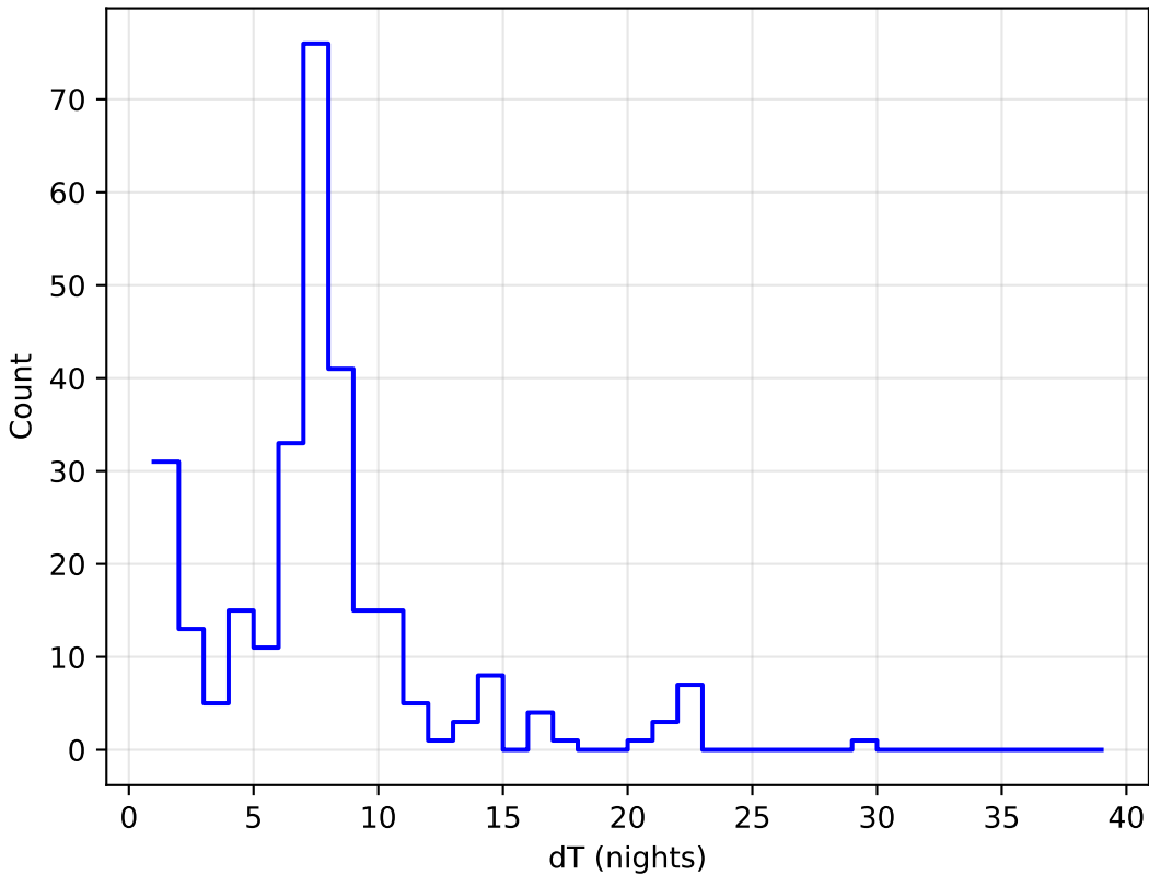
too_100_1v3.4_10yrs all bands: DD:EDFS Delta Nights Histogram
