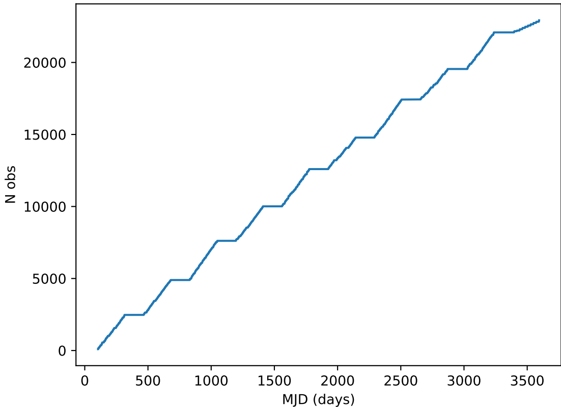
too_100_1v3.4_10yrs all bands: DD:EDFS Cumulative NVisits
