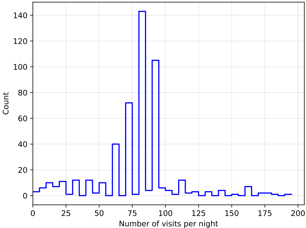
too_100_1v3.4_10yrs all bands: DD: COSMOS NVisitsPerNight
