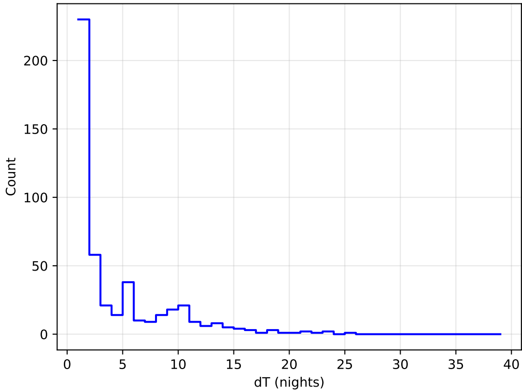
too_100_1v3.4_10yrs all bands: DD:COSMOS Delta Nights Histogram
