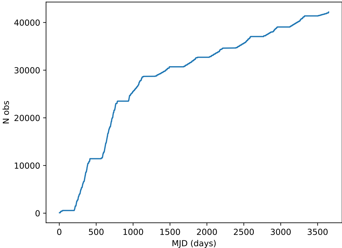
too_100_1v3.4_10yrs all bands: DD: COSMOS Cumulative NVisits
