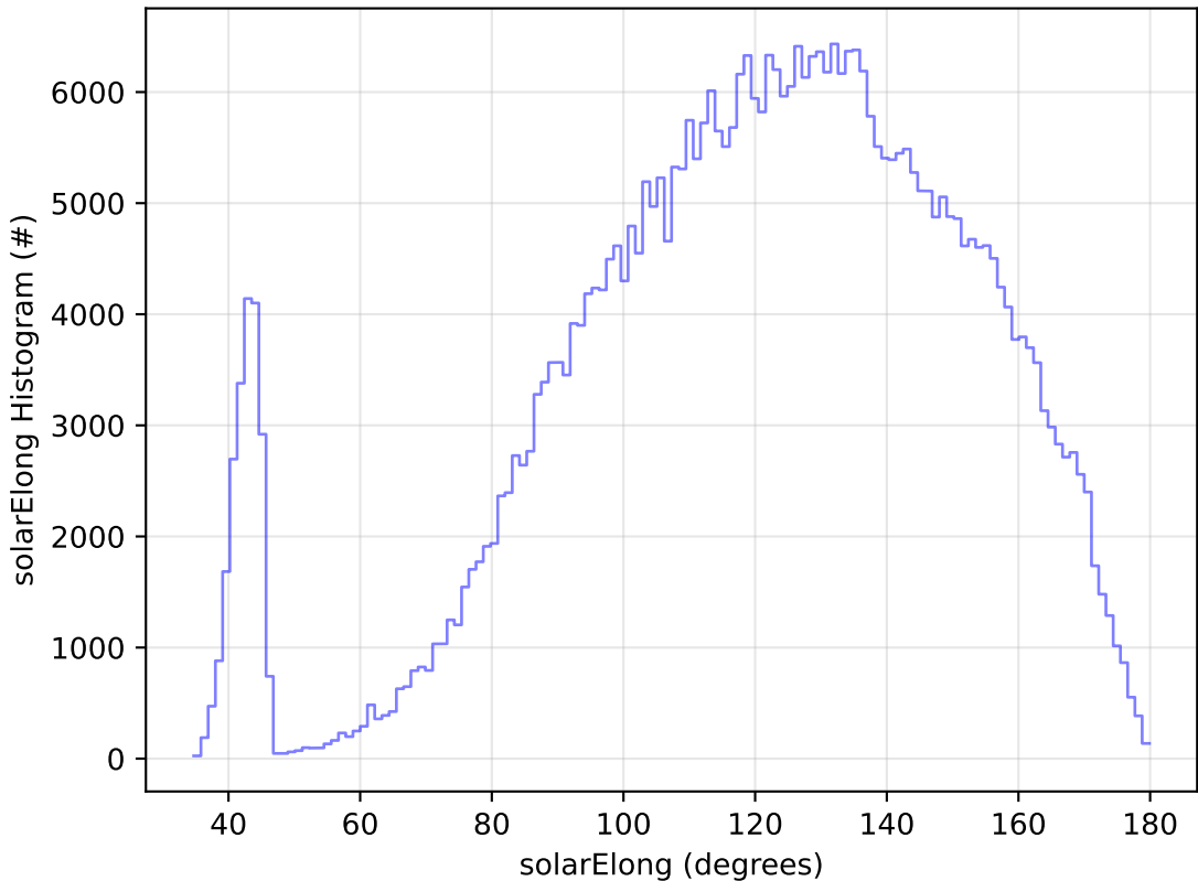
telescope_jerk_v3.5_10yrs WFD z band: solarElong Histogram
