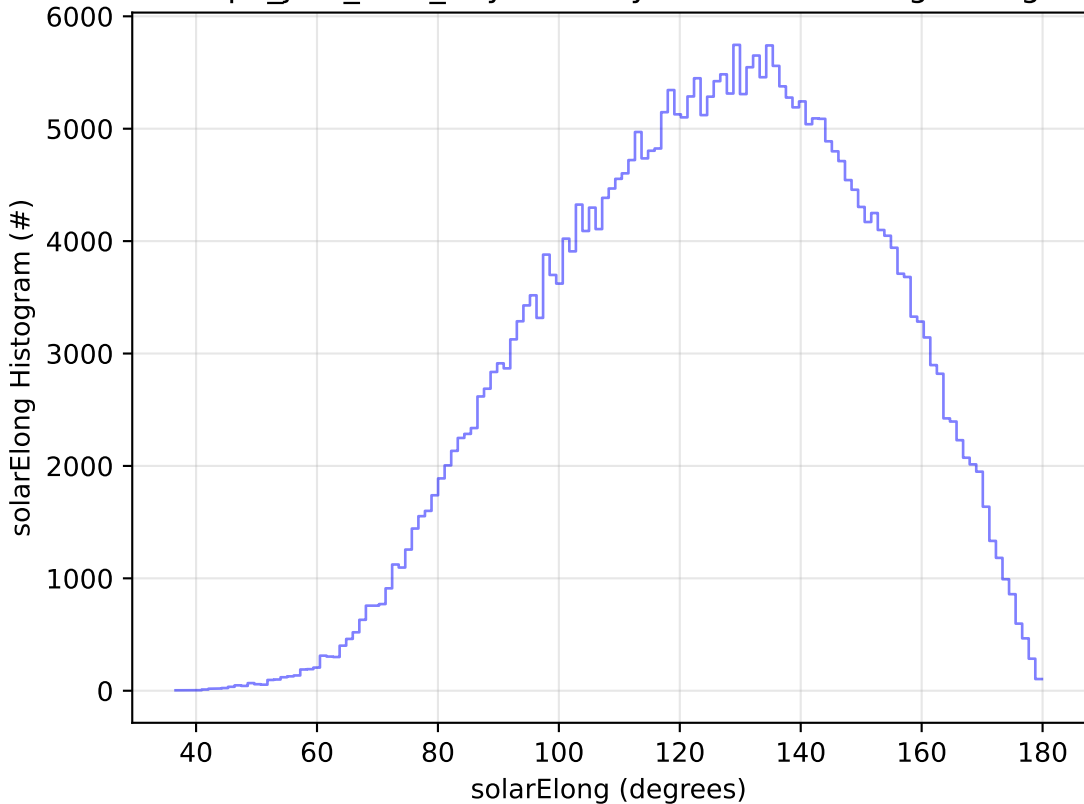
telescope_jerk_v3.5_10yrs WFD y band: solarElong Histogram
