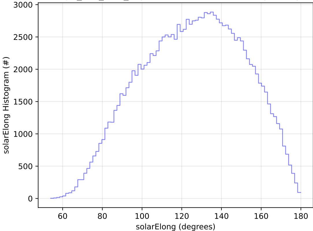
telescope_jerk_v3.5_10yrs WFD u band: solarElong Histogram
