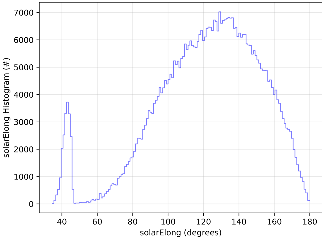
telescope_jerk_v3.5_10yrs WFD r band: solarElong Histogram
