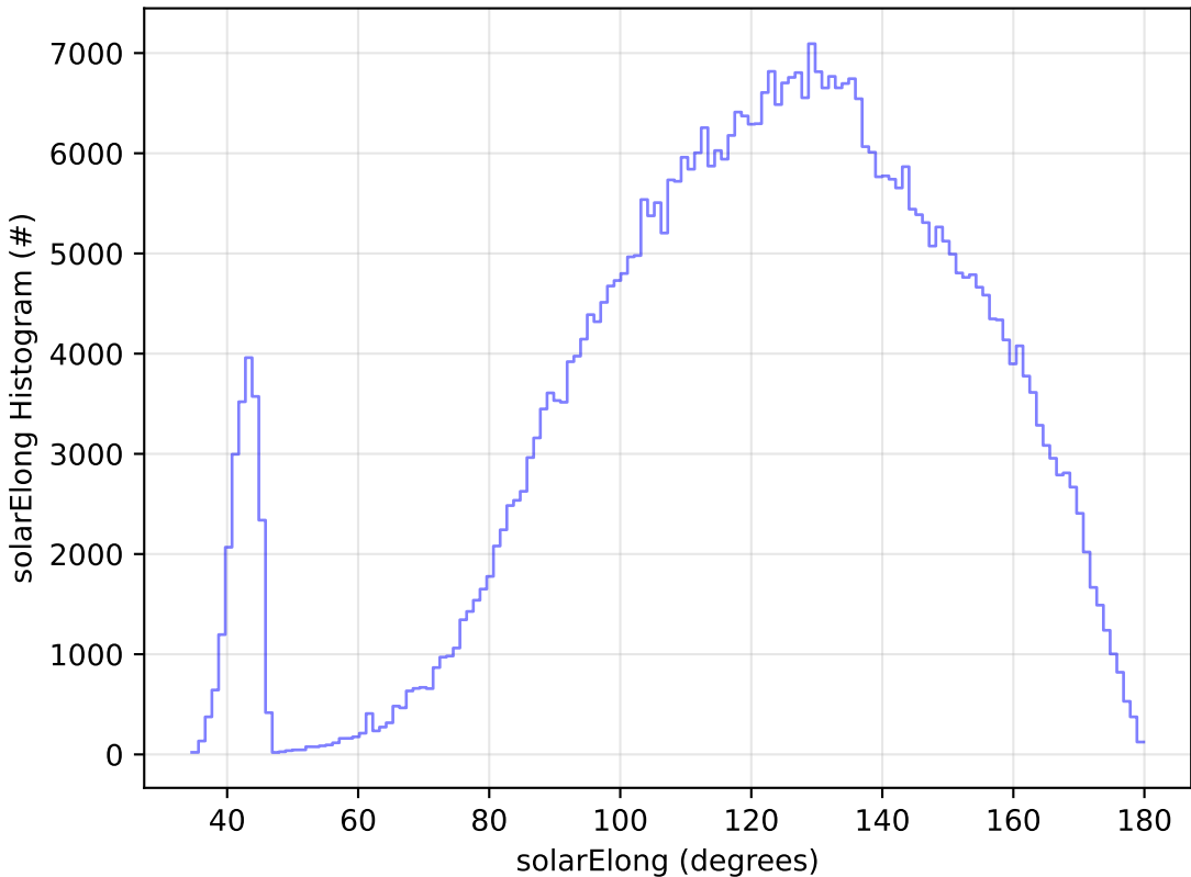
telescope_jerk_v3.5_10yrs WFD i band: solarElong Histogram
