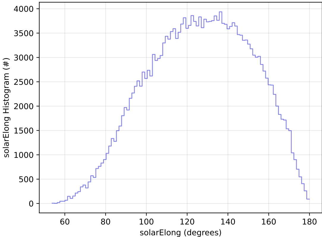
telescope_jerk_v3.5_10yrs WFD g band: solarElong Histogram
