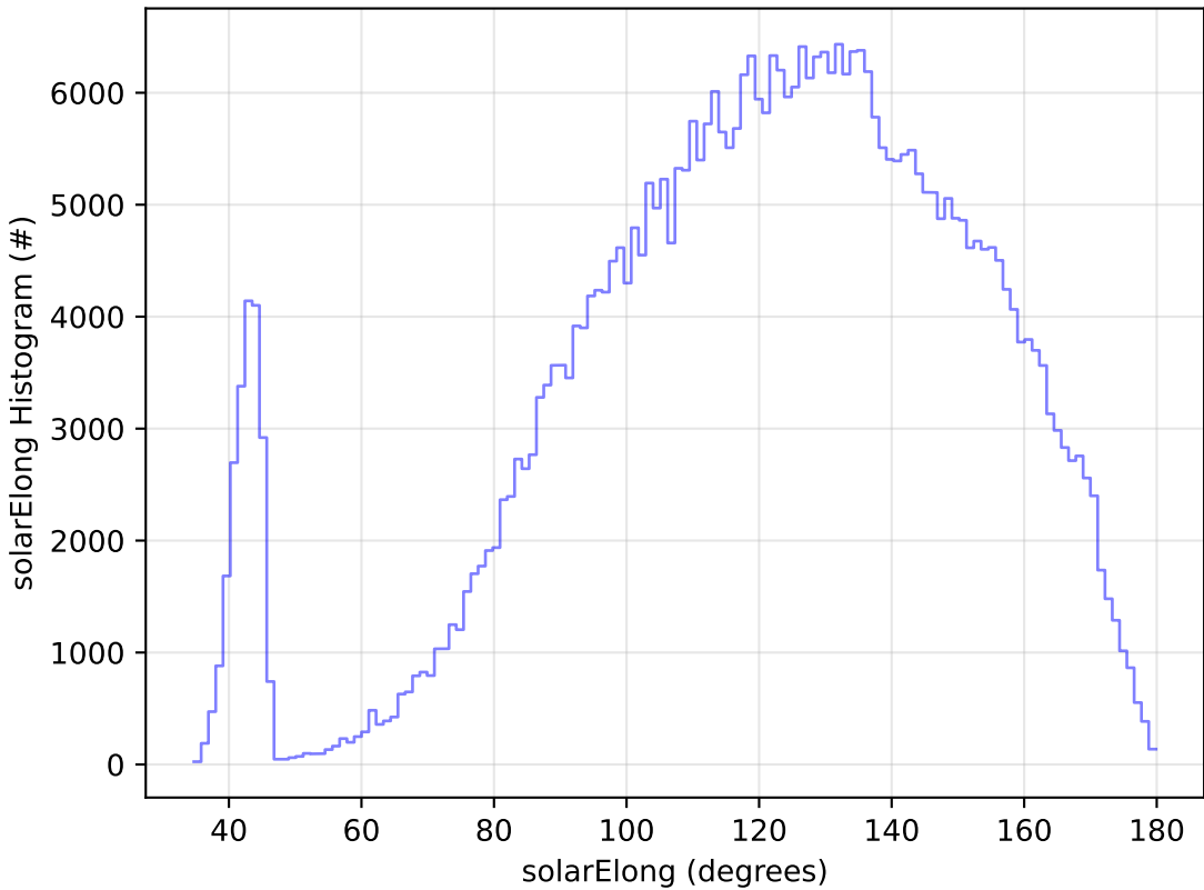
telescope_jerk_v3.5_10yrs All sky z band: solarElong Histogram
