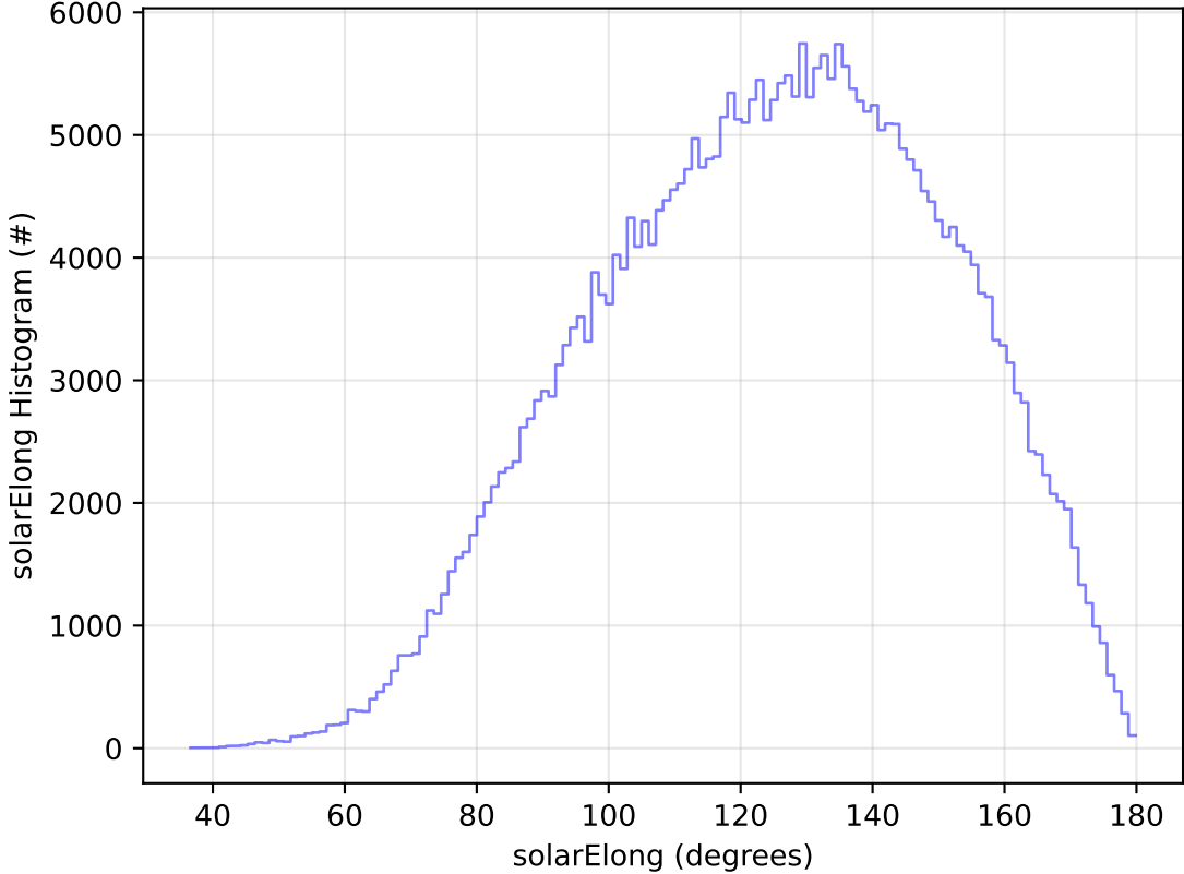
telescope_jerk_v3.5_10yrs All sky y band: solarElong Histogram
