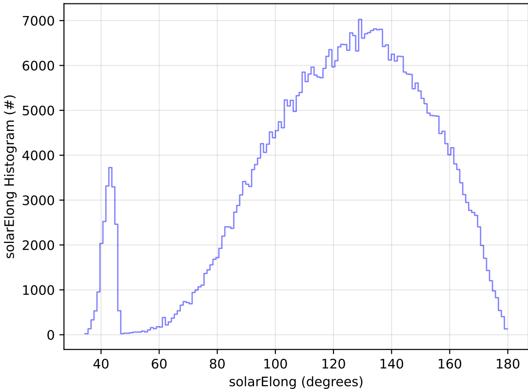
telescope_jerk_v3.5_10yrs All sky r band: solarElong Histogram
