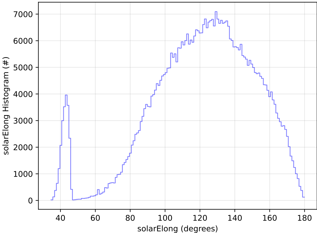
telescope_jerk_v3.5_10yrs All sky i band: solarElong Histogram
