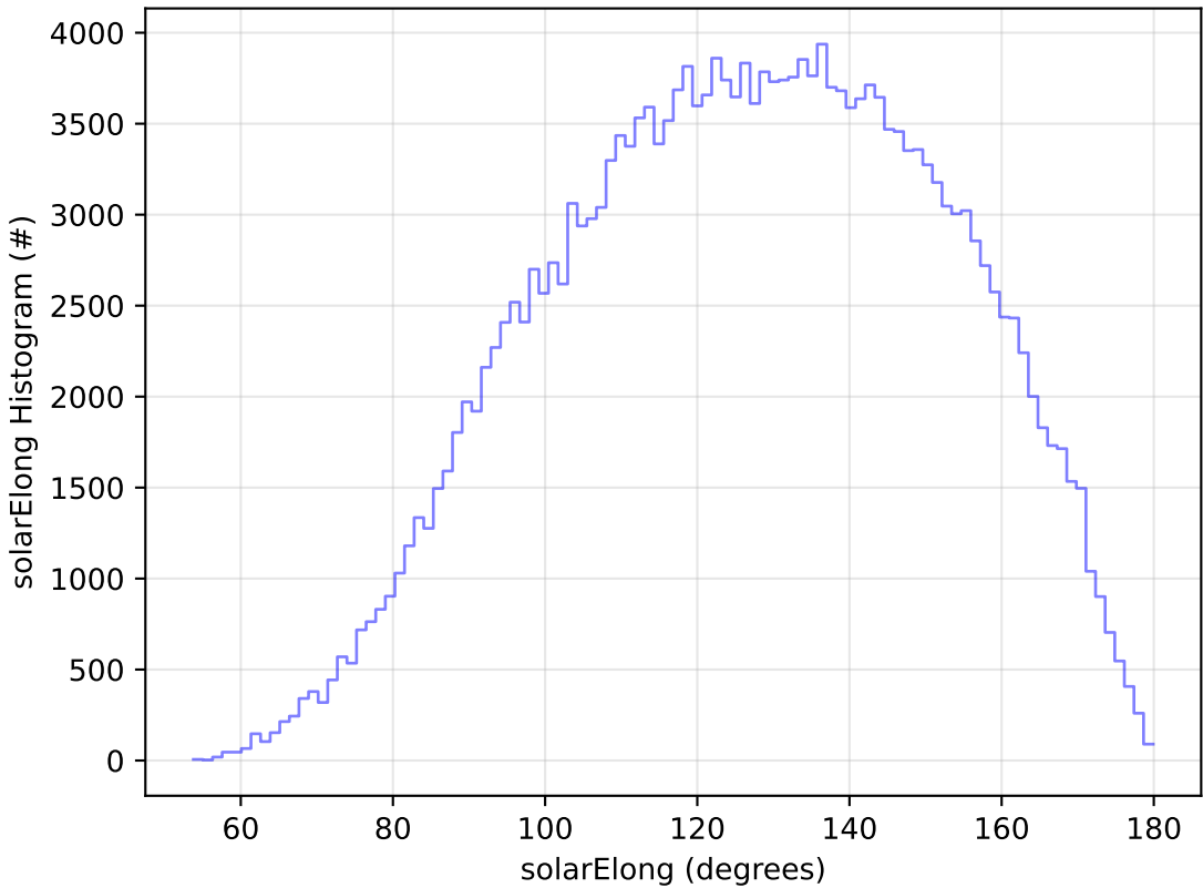
telescope_jerk_v3.5_10yrs All sky g band: solarElong Histogram
