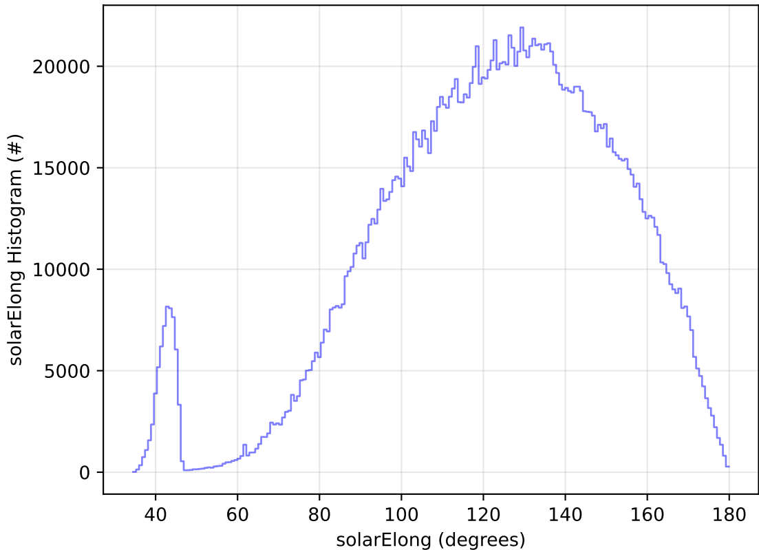
telescope_jerk_v3.5_10yrs All sky all bands: solarElong Histogram
