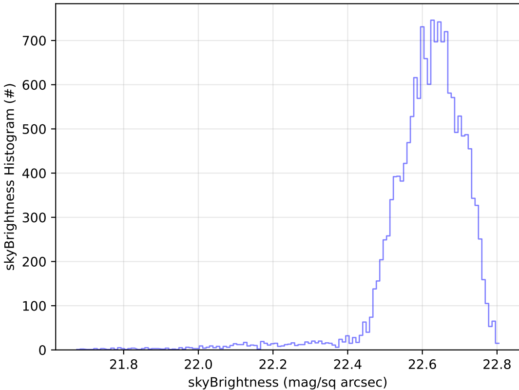
telescope_jerk_v3.5_10yrs Yr 1 u band: skyBrightness Histogram
