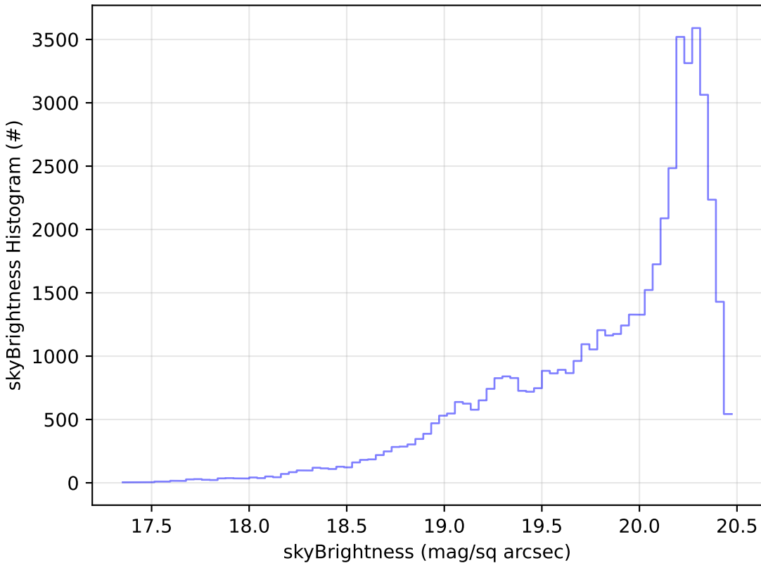
telescope_jerk_v3.5_10yrs Yr 1 i band: skyBrightness Histogram
