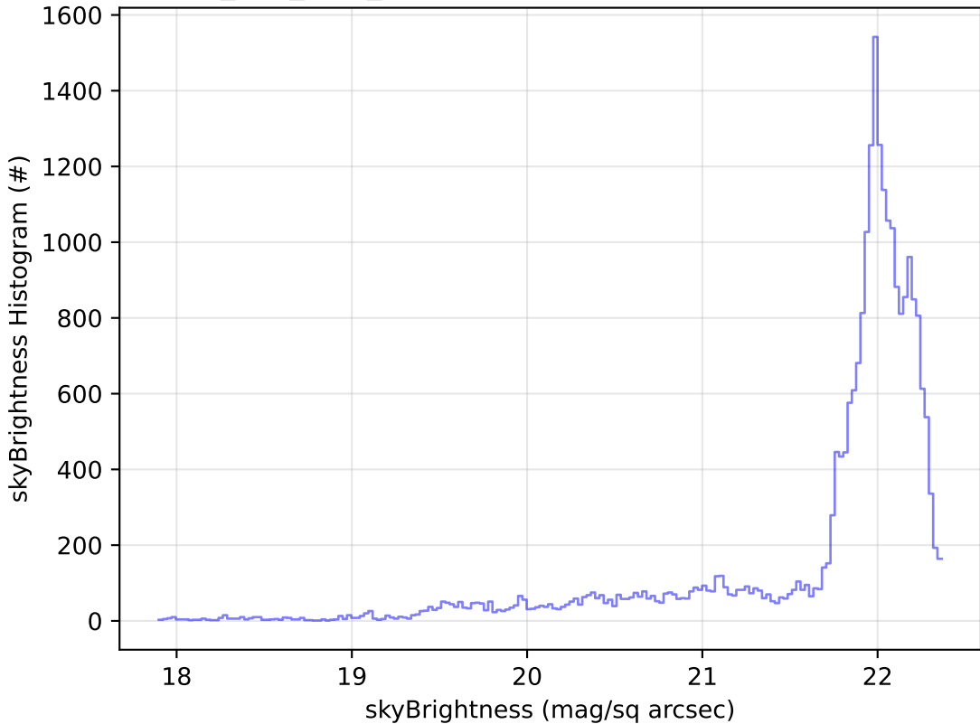
telescope_jerk_v3.5_10yrs Yr 1 g band: skyBrightness Histogram
