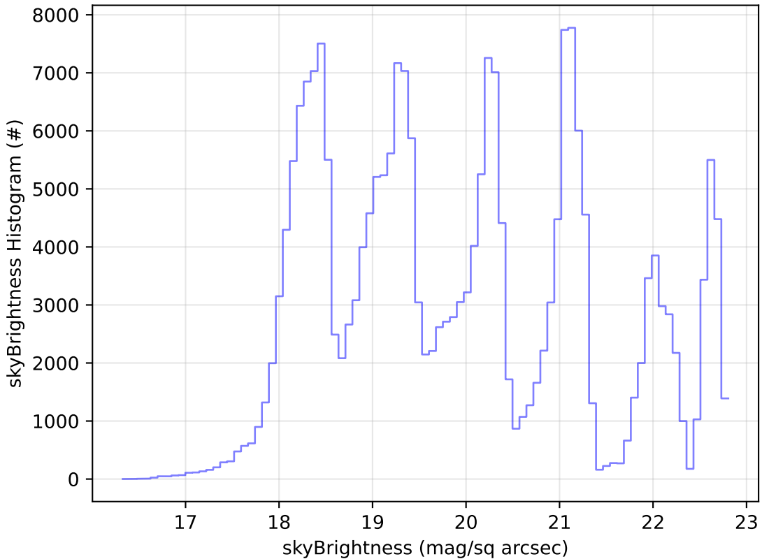
telescope_jerk_v3.5_10yrs Yr 1 all bands: skyBrightness Histogram
